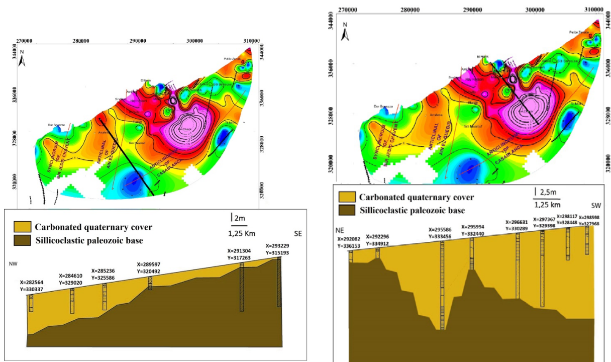
Fig. 5 Map of the isobaths of the surface of the Paleozoic basement of Casablanca
