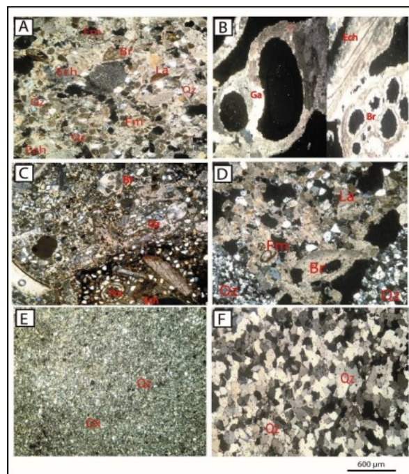
Fig. 4 Microphotographs of thin sections of the main petrographic facies composing the soil of Casablanca. A: Calcarenité, B: Lumachelle, C: Lumachellic sandstone, D: Conglomerate, E: Schist, F: Quartzite
