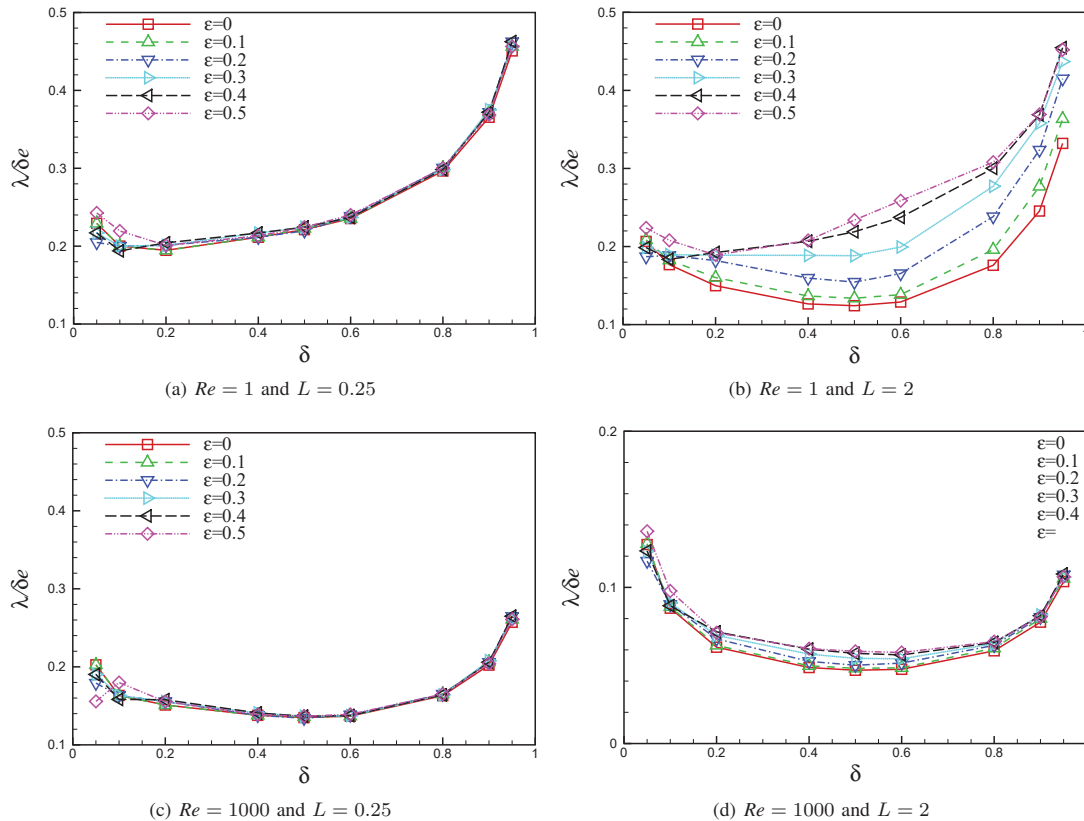
Fig. 5 The effect of the fraction of slip space \delta on the slip length \lambda/\delta e at Re = 1, 1000 and L = 0.25, 2
