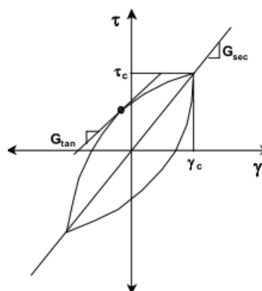
(a) Hysteresis loop
