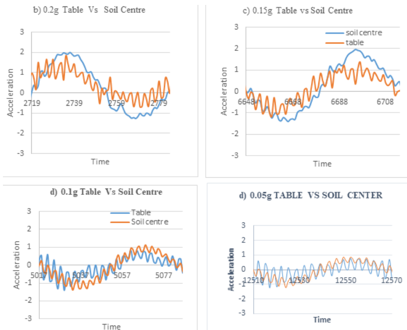
Fig. 12 Soil response
