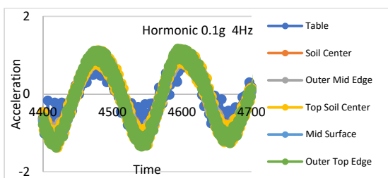
Fig. 9 The effect of the container boundary of the soil
