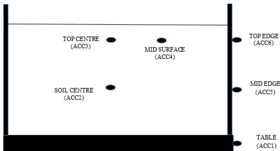
Fig. 5 Acceleration layout
