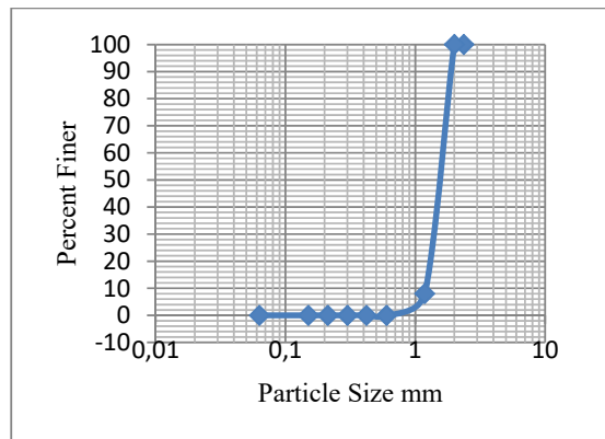
Fig. 3 Selected Soil
