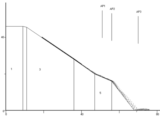
Fig. 5 Cutting 14039: Rock fall model output for 0.8 m diameter boulder with starting velocity H = 0.95 m/s, V = - 0.95 m/s
