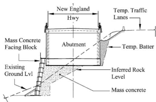
Fig. 3 (b) Typical elevation of abutment retaining wall
