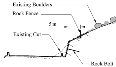
Fig. 6 Rock fence with new cut and upslope
