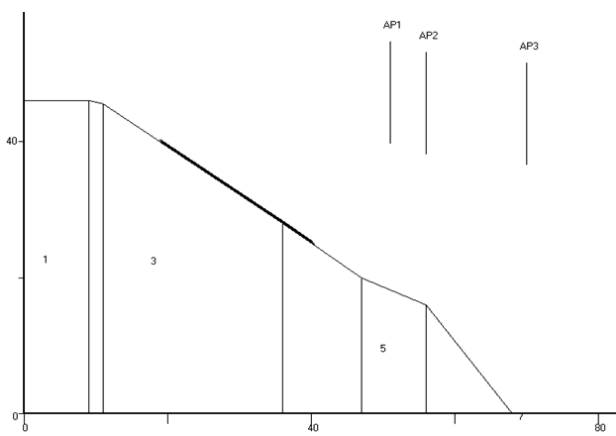
Fig. 4 Cutting 14039: Rock fall model output for 0.8 m diameter boulder with starting velocity H = 0.8 m/s, V = - 0.8 m/s
