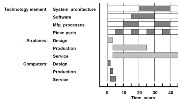
Fig. 1 Component technology, airplane, and computer lifetimes [4]
