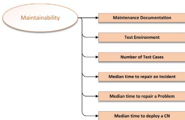
Fig. 8 Maintainability Indicators
