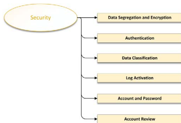
Fig. 9 Security Indicators
