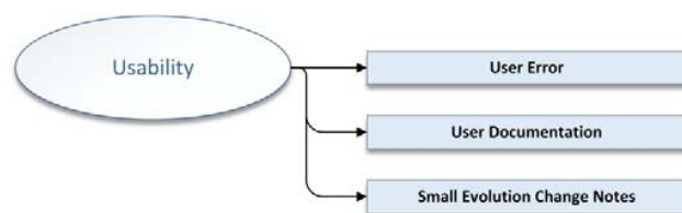
Fig. 7 Usability Indicators
