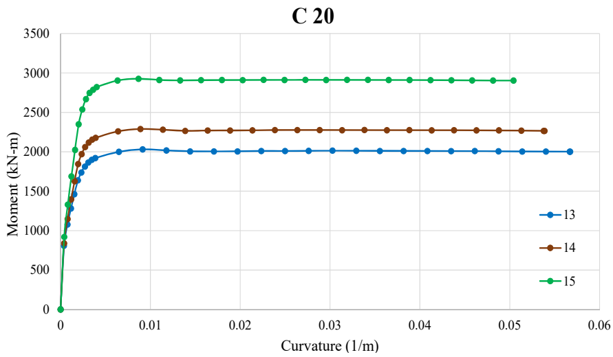
Fig. 7 (a) MC relationship with longitudinal reinforcement type
