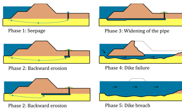
Fig. 1 Backward erosion piping [12]
