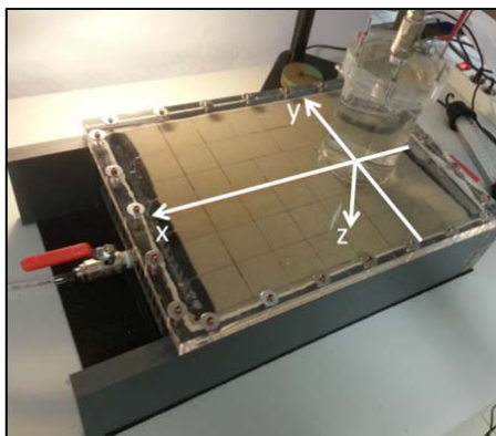
Fig. 2 Test set-up
