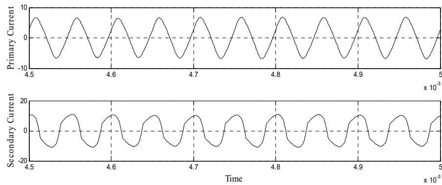
Fig. 10 Primary and secondary currents
