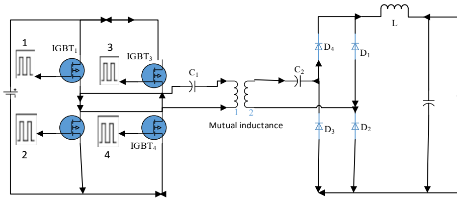
Fig. 8 Simulated circuit
