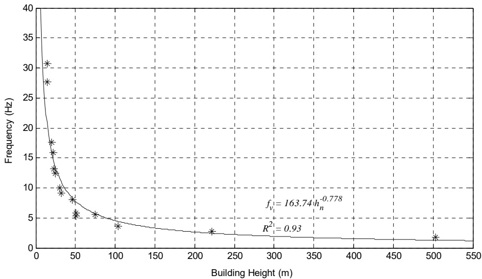
Fig. 8 Natural frequency of vertical
