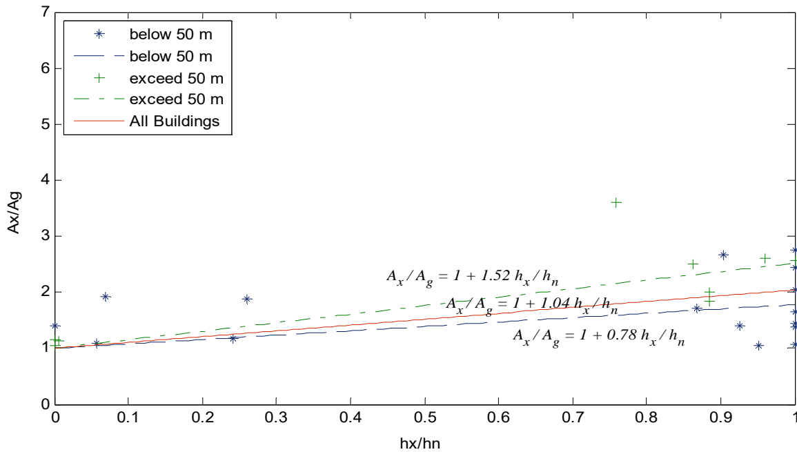
Fig. 4 Floor amplification factor of vertical acceleration
