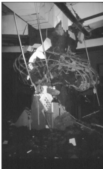
Fig. 2 The failure of column
