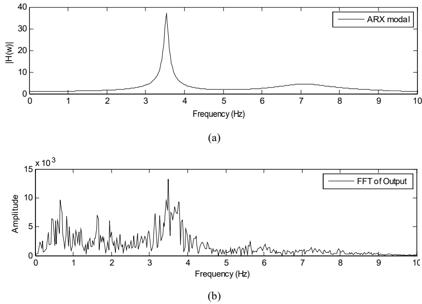
Fig. 7 The signal of input and output (a) ARX model curve (b) FFT output of top floor
