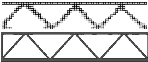
Fig. 11 Skeleton and the corresponding boom
