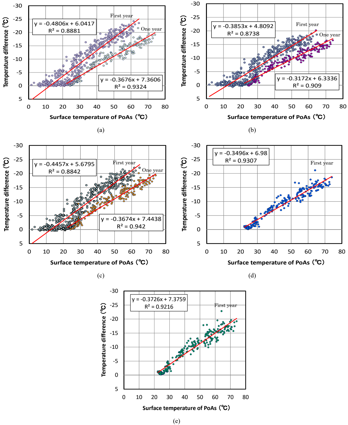
Fig. 4 Surface temperature difference between each specimen and the PoAs (a) JGZ, (b) JGZ-Red, (c) JGZ-Yellow, (d) JGZ-Blue, and (e) JGZ-Green
