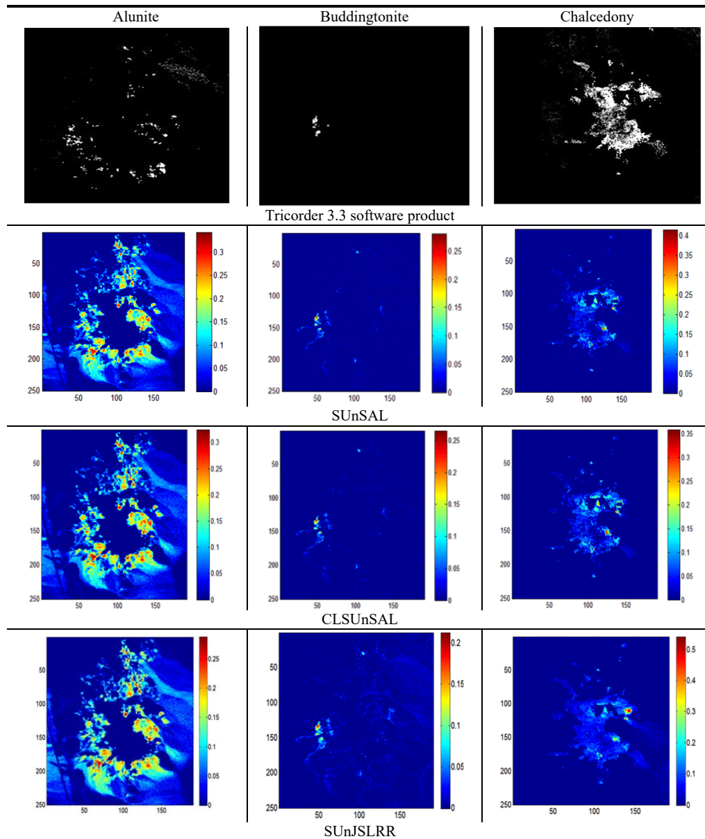
Fig. 2 Abundance maps estimated for the minerals: alunitite , buddingtonite , and chalcedony by applying the different algorithms
