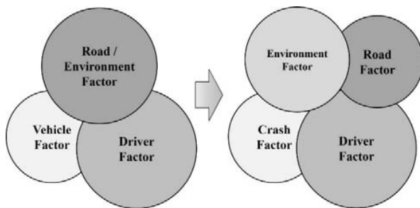
Fig. 1 Latent Factors
