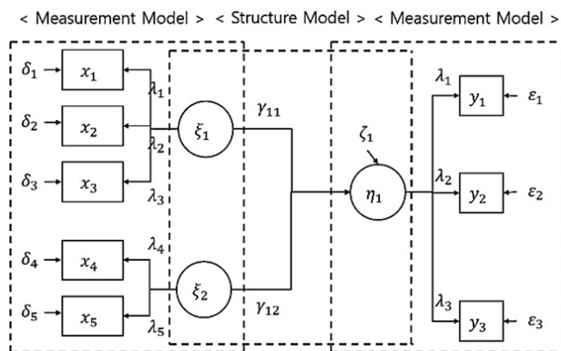
Fig. 2 Structure Map
