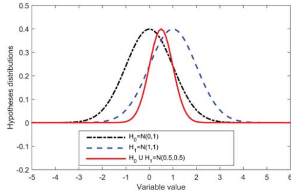
Fig. 2 Hypotheses distributions including null, alternative and uncertainty
