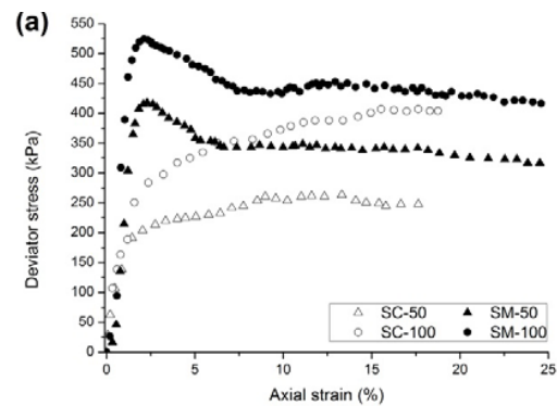
Fig. 4 (a) Deviatoric stress-strain curves, (b) volumetric strain-strain curves, and (c) suction-strain curves of CW tests at the initial matric suction of 100 kPa
