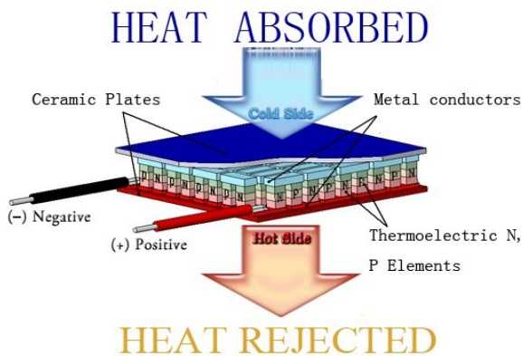
Fig. 1 Peltier chip working function
