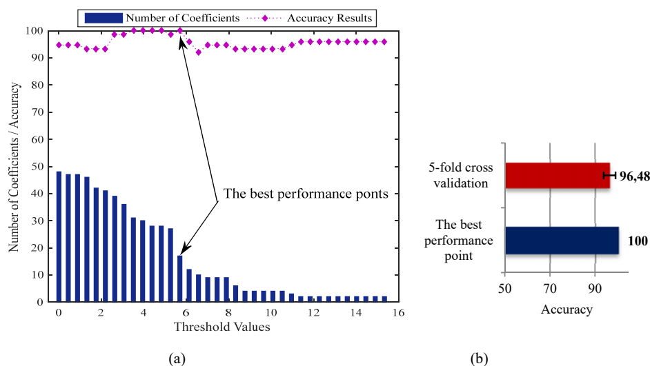
Fig. 2 Normal-abnormal classification for (a) 70-30% ratio of all threshold values (b) 5-fold cross validation
