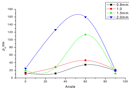
Fig. 7 Test result of the sound pressure for the ultrasonic receiving sensor on the rotation flat
