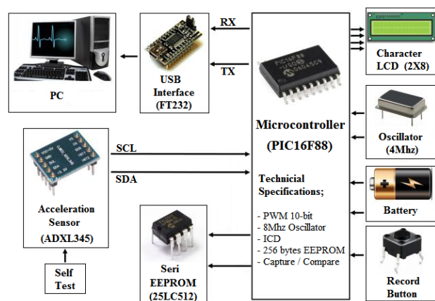
Fig. 4 The block diagram of designed and realized system
