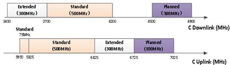
Fig. 2 C band allocation
