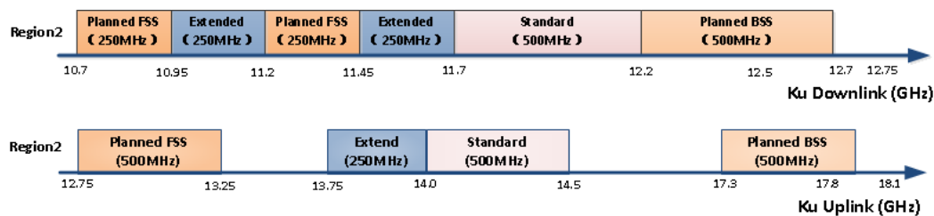
Fig. 3 Ku band allocation
