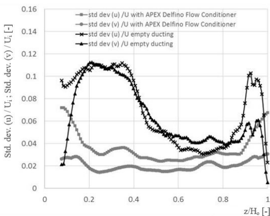
Fig. 4 Profile of normalized standard deviation (normalized with maximum cross sectional velocity in x-direction) at a stream wise position 5h upstream of the inlet into the five channel model with and without Flow Conditioner (installed immediately downstream of the 30 degree ducting)
