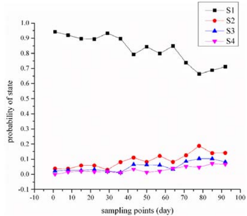
Fig. 3 The probability distribution sequence of the angle state
