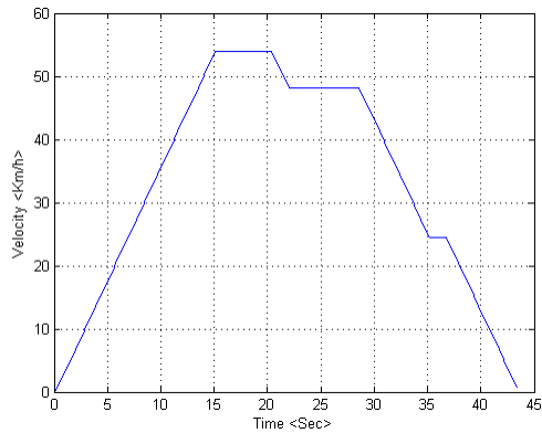
Fig. 6 Simplified Trajectory
