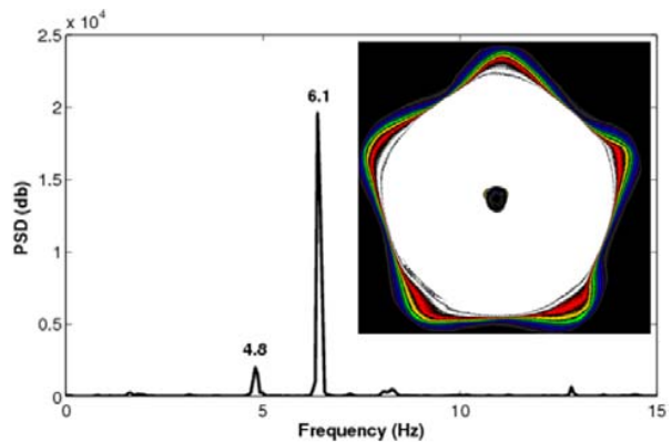
Fig. 9 Pentagonal pattern ( N = 5 ) and corresponding power spectrum
