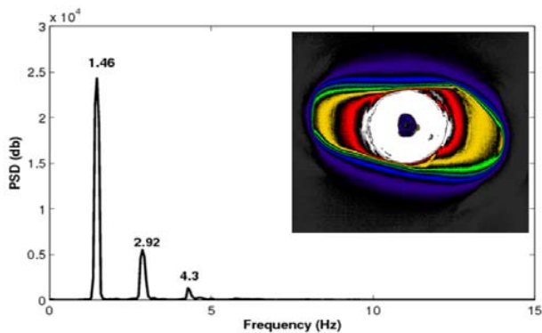
Fig. 3 Elliptical pattern ( N= 2 ) and corresponding power spectrum
