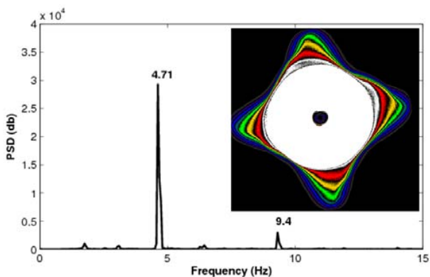
Fig. 7 Square pattern ( N = 4 ) and corresponding power spectrum
