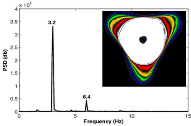
Fig. 5 Triangular pattern ( N = 3 ) and corresponding power spectrum
