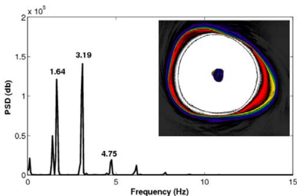
Fig. 4 First transition from N=2 to N=3 and corresponding power spectrum
