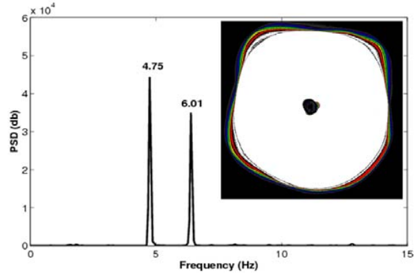
Fig. 8 Third transition from N=4 to N=5 and corresponding power spectrum
