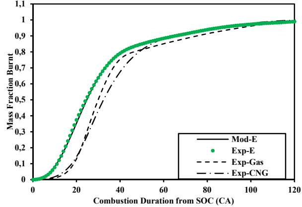
Fig. 8 (e) Comparison of Experimental and dual Wiebe modeled curves of PG Set-E operation at WOT, \Phi=1.13 , rpm=1500 and modeled coefficients x=0.80 , a_1=60 , m_1=1.41 , a_2=5.3 , m_2=1.8
