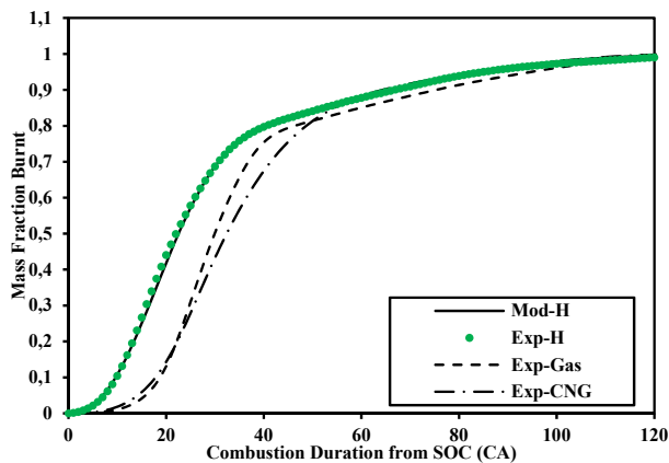
Fig. 8 (h) Comparison of Experimental and dual Wiebe modeled curves of PG Set-H operation at WOT, \Phi=1.18 , rpm=1500 and modeled coefficients \alpha=0.783 , a_1=70 , m_1=1.35 , a_2=5.7 , m_2=1.8
