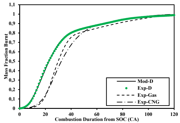
Fig. 8 (d) Comparison of Experimental and dual Wiebe modeled curves of PG Set-D operation at WOT, \Phi=1.15 , rpm=1500 and modeled coefficients x=0.80 , a_1=60 , m_1=1.26 , a_2=6.3 , m_2=1.88
