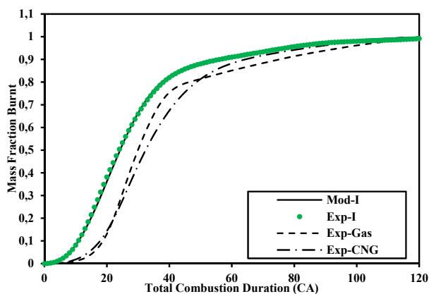
Fig. 8 (i) Comparison of Experimental and dual Wiebe modeled curves of PG Set-I operation at WOT, \Phi=0.97 , rpm=1500 and modeled coefficients \alpha=0.84 , a_1=65 , m_1=1.45 , a_2=6 , m_2=1.8
