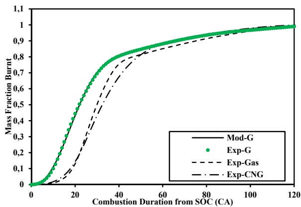
Fig. 8 (g) Comparison of Experimental and dual Wiebe modeled curves of PG Set-G operation at WOT, \Phi=1.15 , rpm=1500 and modeled coefficients \alpha=0.785 , a_1=75 , m_1=1.38 , a_2=5 , m_2=1.7
