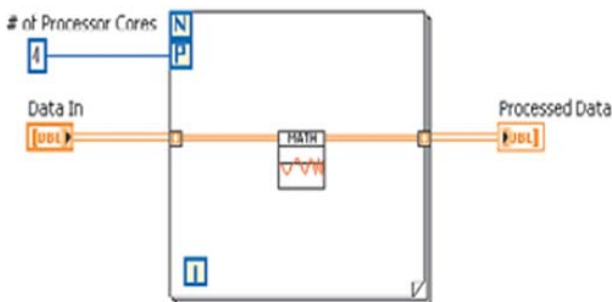
Fig. 5 Example of Parallelism on Loops on LabVIEW [5]
