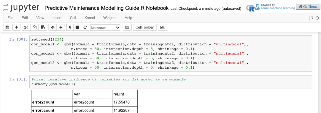
Fig. 7 Using jupyter notebook in Azure
