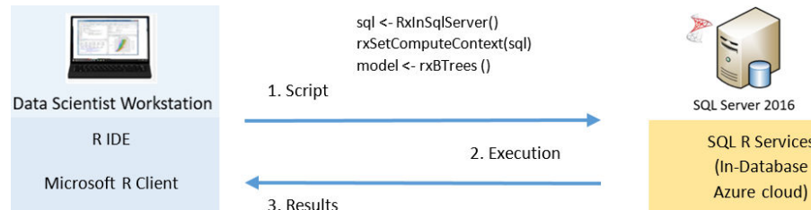
Fig. 4 Cloud based solution framework-2
