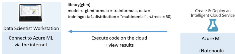
Fig. 3 Cloud based solution framework-1
