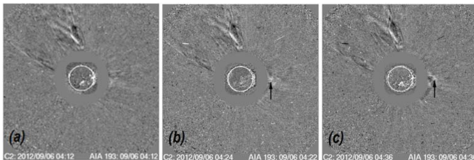
Fig. 2 Image (a) shows solar corona at the peak intensity of the flare. Arrows (b) & (c) mark eruption from the active region. The CME does not appear very prominent in the coronagraph images
