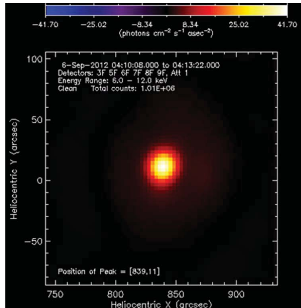
Fig. 1 Reconstructed 6-12 keV energy band RHESSI image
