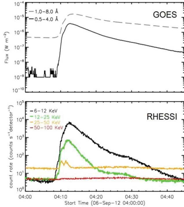
Fig. 3 The GOES time profiles are obtained for 1.0-8.0 Å (12.5-1.5 keV) and 0.5-4.0 Å (24.0-3.0 keV) SXR channels. The RHESSI time profiles are obtained for energy bands of 6-12 keV, 12-25 keV, 25-50 keV, and 50-100 keV
