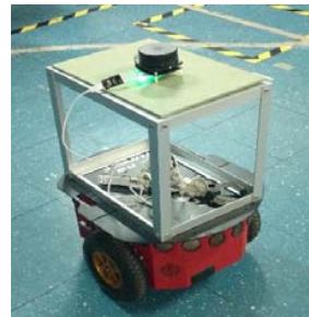
Fig. 6 Mobile robot (Pioneer 3DX) and RPLIDAR (black disc on top) as part of the N-MARIA structure
