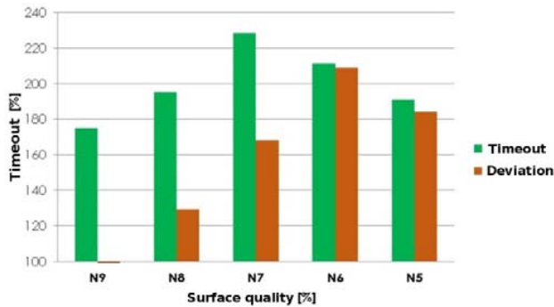
Fig. 3 Relationship of surface quality and setup time
