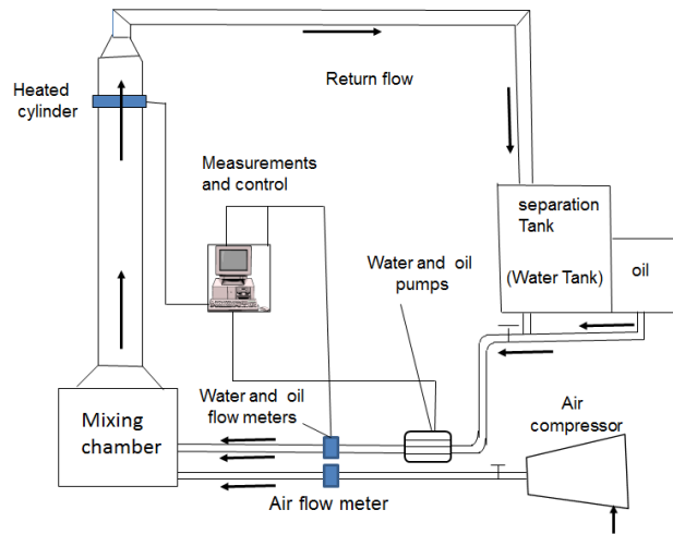
Fig. 1 Schematic diagram of experimental facility
