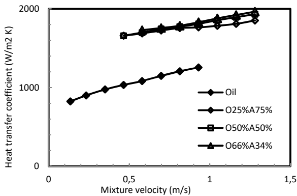
Fig. 5 Variation of average heat transfer coefficient with mixture velocity of oil-air two-phase flow
