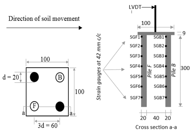
Fig. 5 Details of model piles and cap
