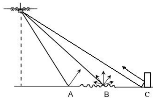
Fig. 7 Backscattering from different surfaces
