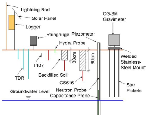
Fig. 5 Schematic of instruments at site [25]
