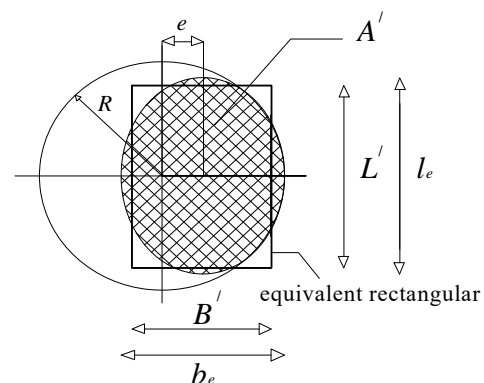
Fig. 1 Effective area method [2]
