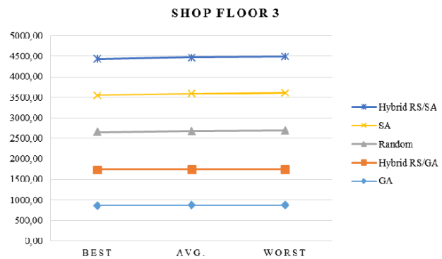
Fig. 8 Results of Shop Floor 3
