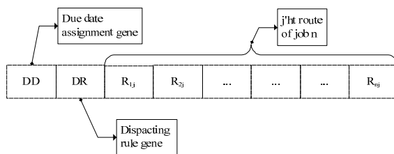
Fig. 1 Chromosome representation
