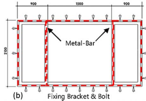
Fig. 2 Two windows model (a) window considered one panel, and (b) window considered three separate panels
