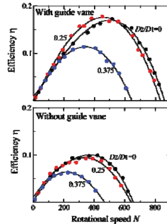
Fig. 8 Effect of hollow ratio on turbine efficiency
