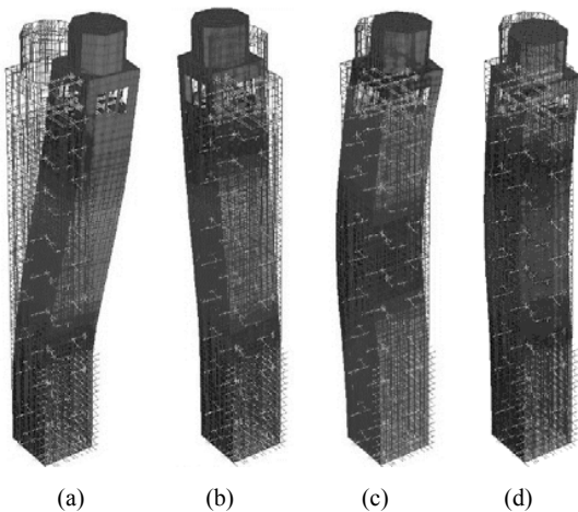
Fig. 14 Modal shapes obtained from Model 2
