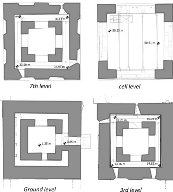
Fig. 3 Frari bell tower, plans
