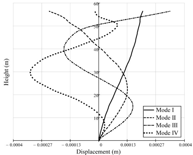
Fig. 13 Displacement evaluation on Model 1
