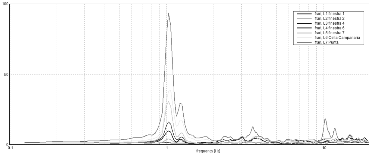
Fig. 7 Frequency peaks
