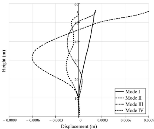
Fig. 15 Displacement evaluation on Model 2
