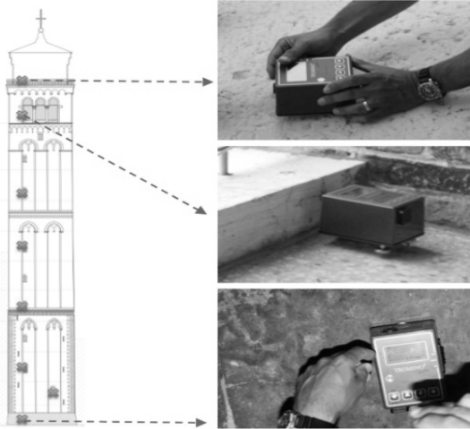
Fig. 4 Tromograph placements
