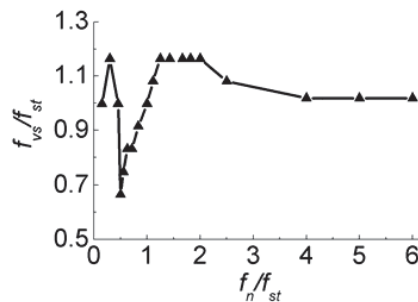
Fig. 4 (c) frequency of vortex shedding versus f_n/f_{st}
