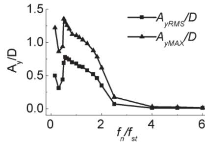
Fig. 4 (b) Lateral amplitude versus f_n/f_{st}
