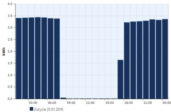
Fig. 9 Energy consumed daily by the street lighting – example
