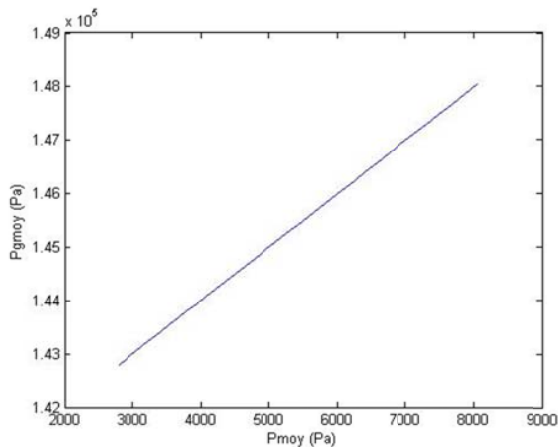
Fig. 16 Variation of P_{gmoy} with P_{moy}
