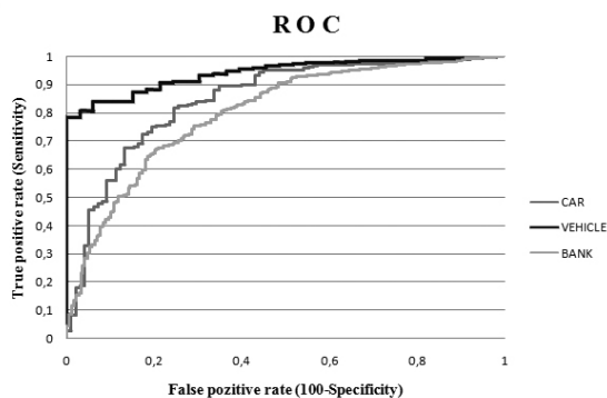
Fig. 3 ROC curves
