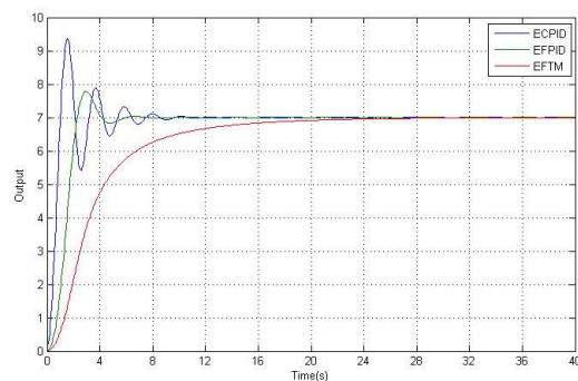
Fig. 8 Step responses for input with amplitude 7
