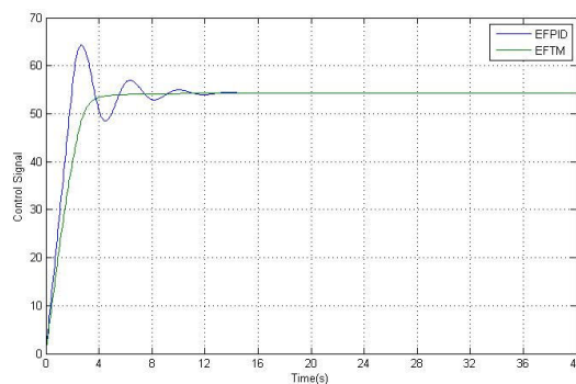
Fig. 14 Control signals for input with amplitude 12
