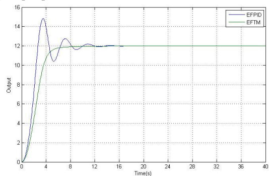
Fig. 12 Step responses for input with amplitude 12
