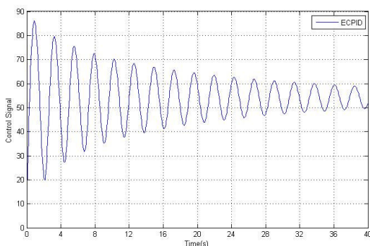
Fig. 15 Control signal for input with amplitude 12 (ECPID)
