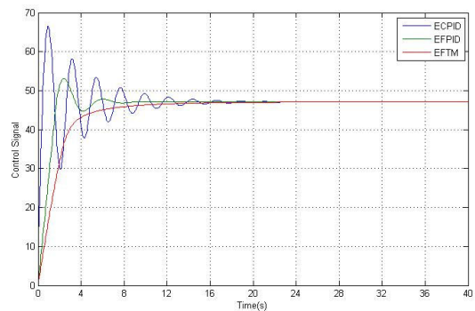
Fig. 11 Control signals for input with amplitude 9
