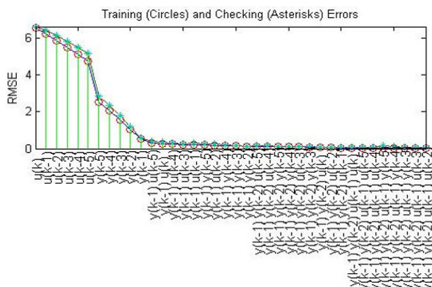
Fig. 4 Best input set obtained by ANFIS
