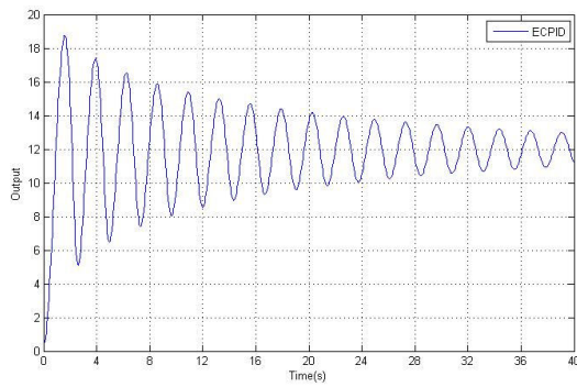
Fig. 13 Step response for input with amplitude 7 (ECPID)
