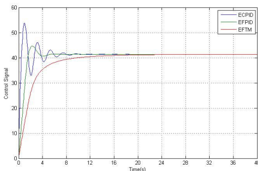
Fig. 9 Control signals for input with amplitude 7
