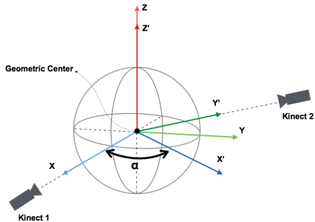
Fig. 7 Determine virtual coordinates for Kinect2
