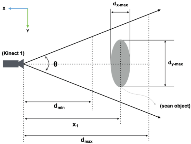
Fig. 4 Relationship between distance of Kinect1 along X-axis and the width of object on Y-axis
