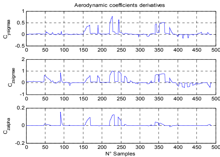
Fig. 6 Aerodynamic coefficients derivatives
