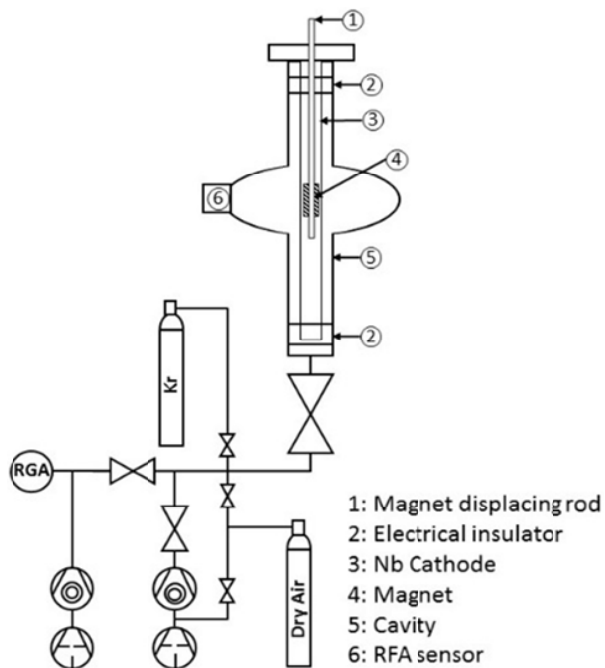
Fig. 2 Schematic of the SRF cavities coating apparatus
