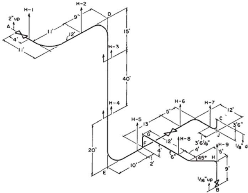
Fig. 1 Piping Routing with Hanger Supports
