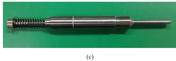
Fig. 5 Upper part of mock-up fuel rod with LVDT core (a) Schematic diagram, (b) Composition, (c) Assembled LVDT core
