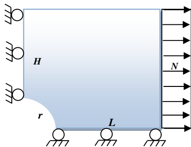
Fig. 5 The infinite plate with a central hole
